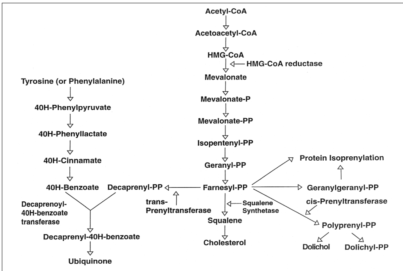
Figure 1. Reaction pathway of the biosynthesis of coenzyme Q 10 (ubiquinone), cholesterol, and dolichols. HMG-CoA = 3-hydroxy-3-methylglutaryl coenzyme A, (PP = pyrophosphate)
